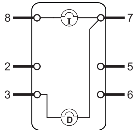
LIGHTING DIAGRAM
